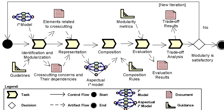
Fig. 1 – The modular i^* with aspects strategy.
