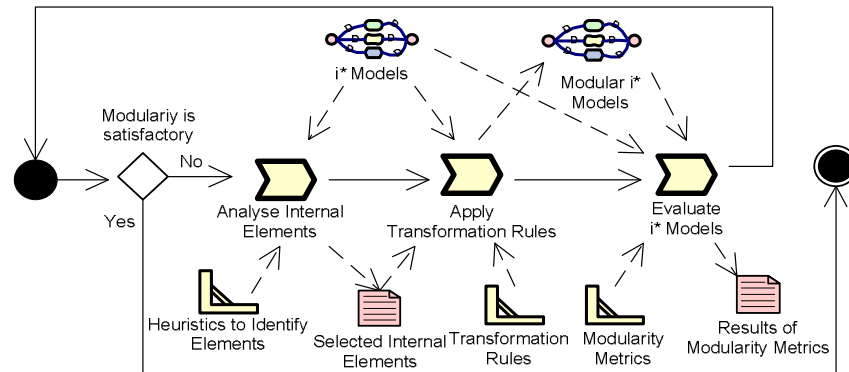
Fig. 2 – The modular i* with model transformation.
