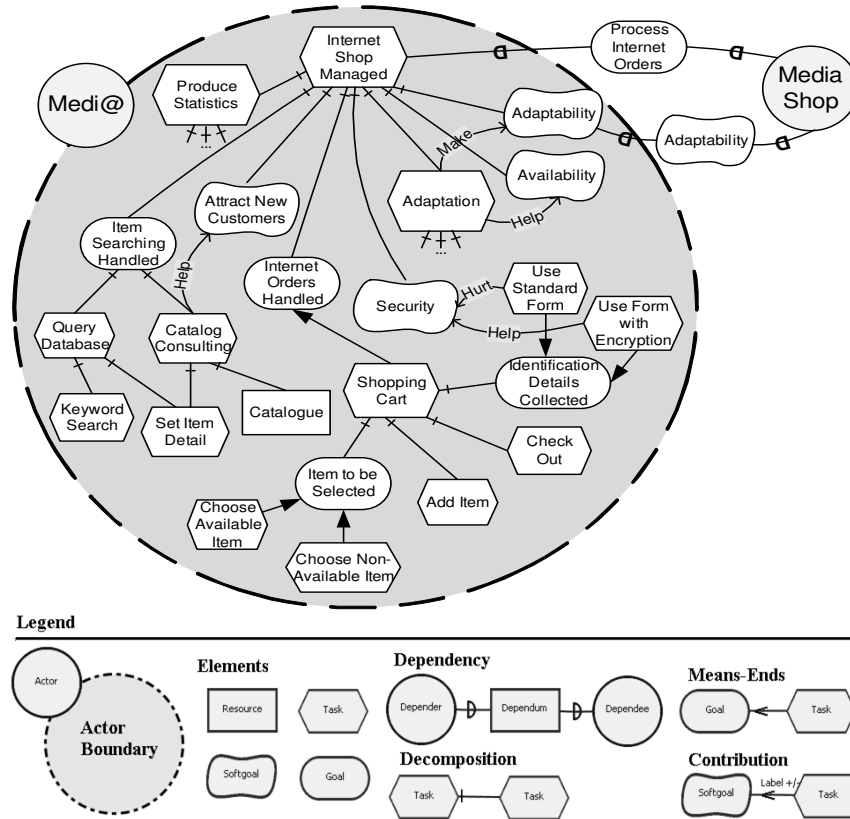
Fig. 3 – SR model for Medi@ system.
